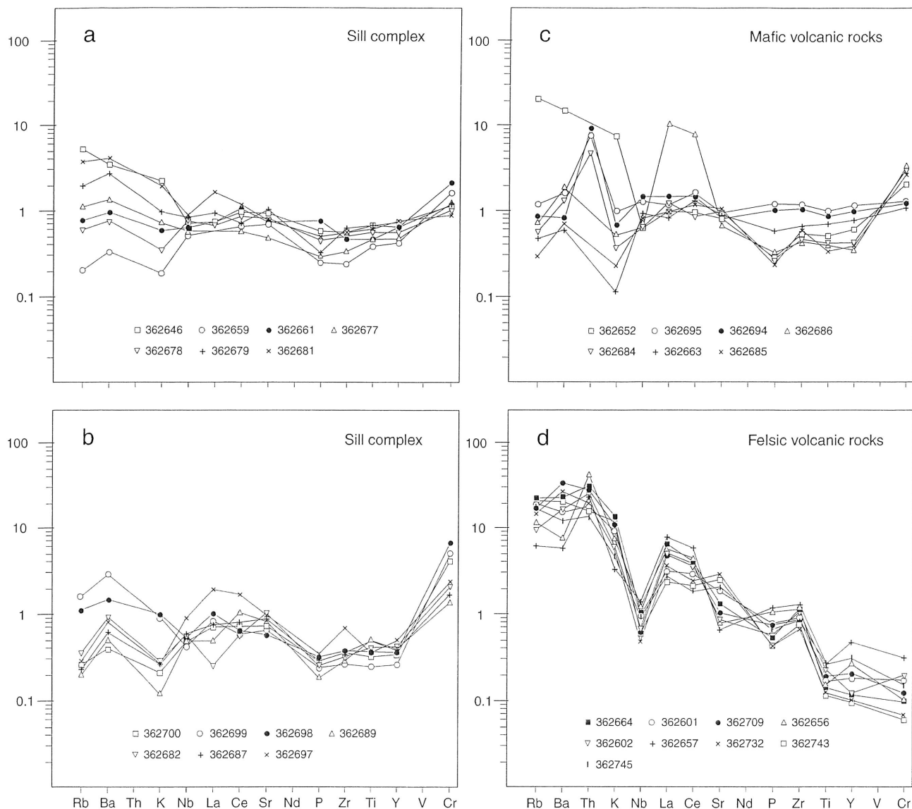
Fig. 5. MORB-normalised multi-element spider diagrams. a and b: Sill complex samples. c: Mafic volcanic samples. d: Felsic volcanic samples. Normalised after Pearce (1983).
