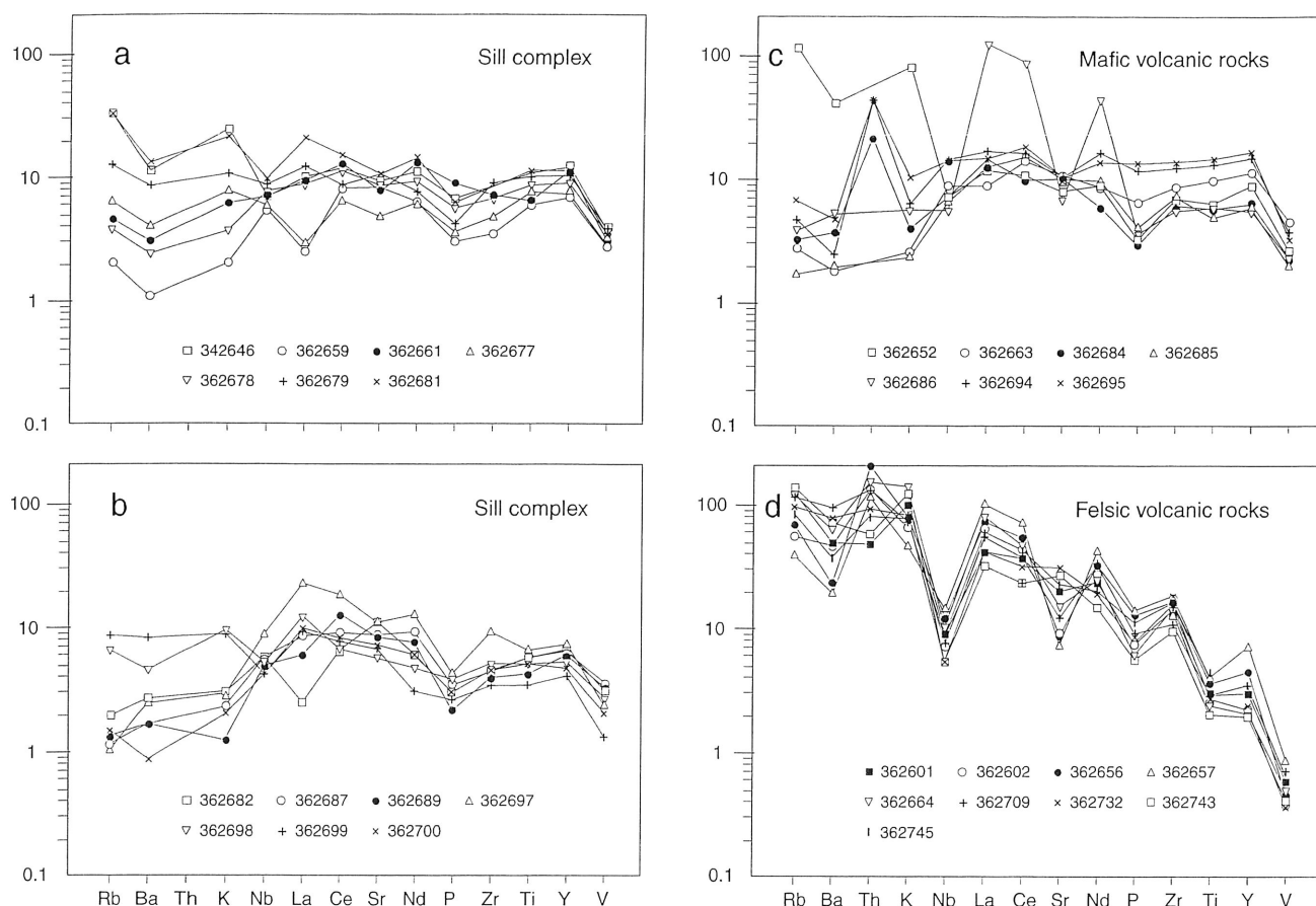
Fig. 4. Chondrite-normalised multi-element spider diagrams for: a and b: Sill complex samples. c: Mafic volcanic samples. d: Felsic volcanic samples. Normalised after Thompson et al. (1984).
