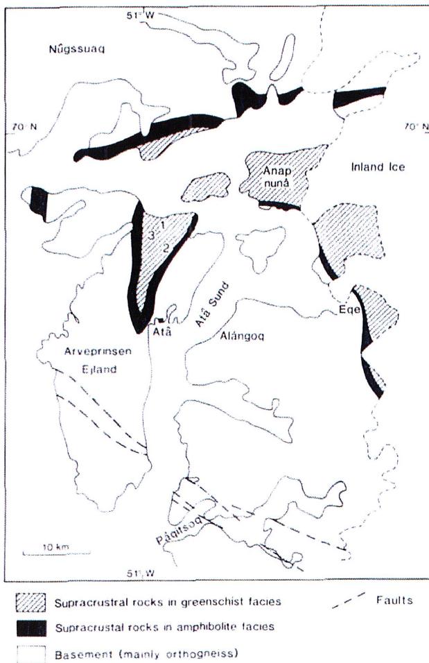
Fig. 1. Generalised geological map of the Atâ area (after Escher & Burri, 1967).
