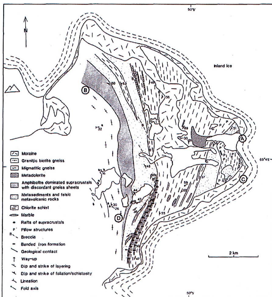
Fig. 4. Geological sketch map of the Ege area.
